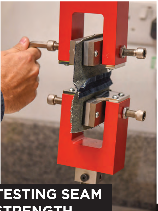
5000KG TENSILE TESTING SYSTEM
